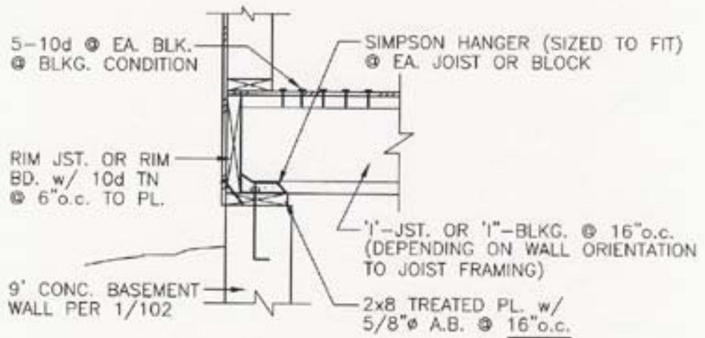
2 CONNECTION OF TOP OF 9'-0" 102 BASEMENT WALL TO FLR. SYSTEM
